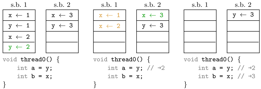
Fig. 3. Suppose thread0 is about to execute with the displayed contents of store buffers of two other threads and suppose it had nondeterministically chosen to load value 2 from y (denoted by green in the figure). The entries at the top of the store buffers are the oldest entries.
